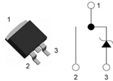
TO-252-2L
