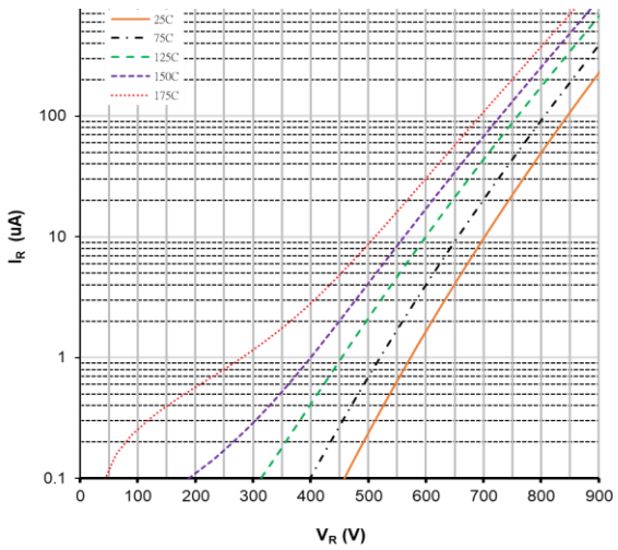
Figure 3. Reverse Characteristics
