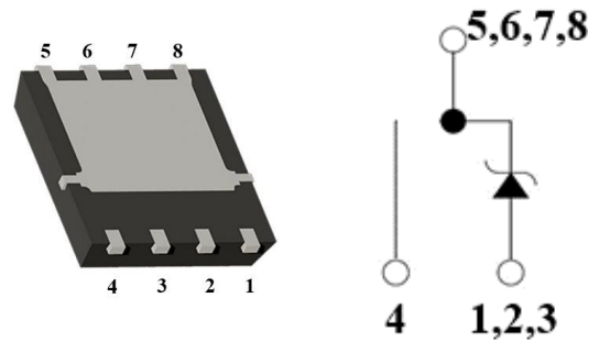
DFN 5x6
