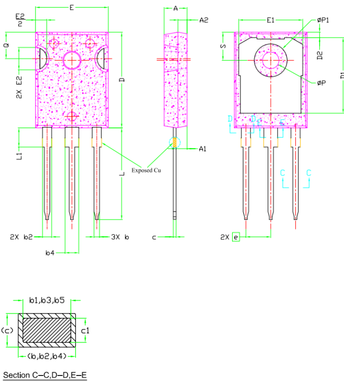
Section C-C, D-D, E-E
